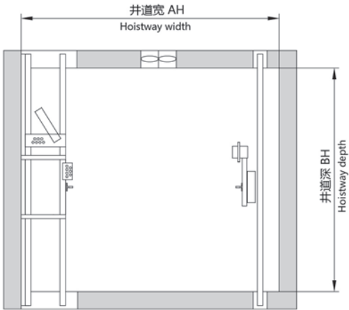
顶部装置布置图 Top of Well layout
